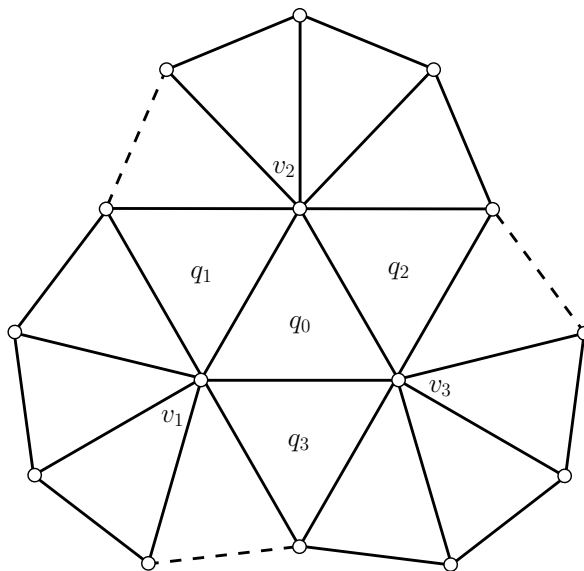
Figure 1: A partial drawing of a local C_d -graph.
